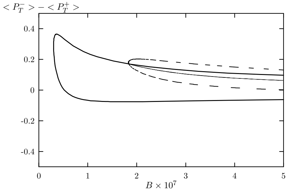
Figure 5: The flows in (\mathcal{B}, \langle P_T^- \rangle - \langle P_T^+ \rangle) plane. In each flow, C_{LL} (thick solid line), C_{LR} (thick dashed line), C_{RL}, C_{RR} (thin solid line) are varied respectively.
