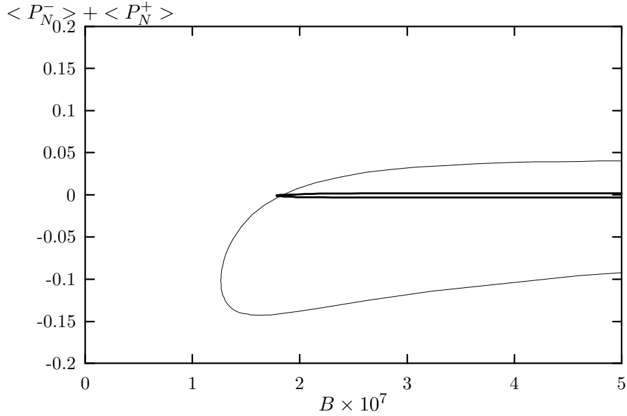
Figure 8: The flows in (\mathcal{B}, \langle P_N^- \rangle + \langle P_N^+ \rangle) plane. In each flow, C_T + 2C_{TE} (thick solid line), C_T - 2C_{TE} (thin solid line) are varied respectively.
