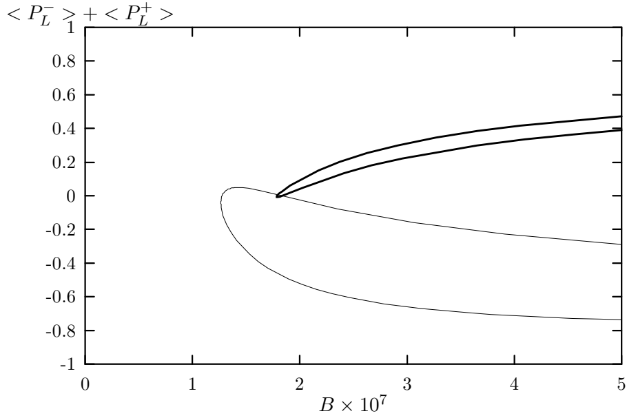
Figure 4: The flows in (\mathcal{B}, \langle P_L^- \rangle + \langle P_L^+ \rangle) plane. In each flow, C_T + 2C_{TE} (thick solid line), C_T - 2C_{TE} (thin line) are varied respectively.
