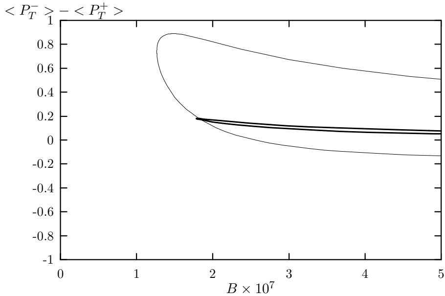
Figure 7: The flows in (\mathcal{B}, \langle P_T^- \rangle - \langle P_T^+ \rangle) plane. In each flow, C_T + 2C_{TE} (thick solid line), C_T - 2C_{TE} (thin solid line) are varied respectively.
