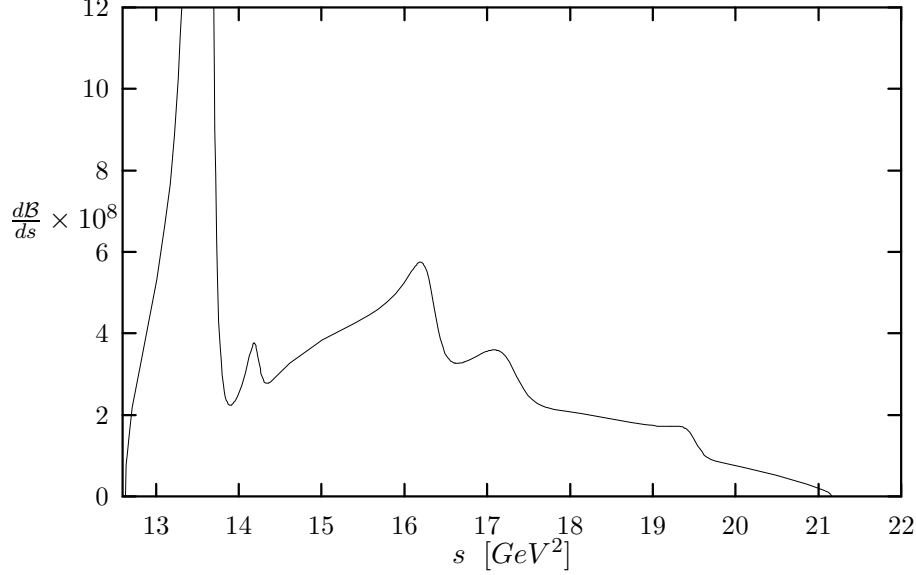
Figure 1: The differential decay rate in the SM.
