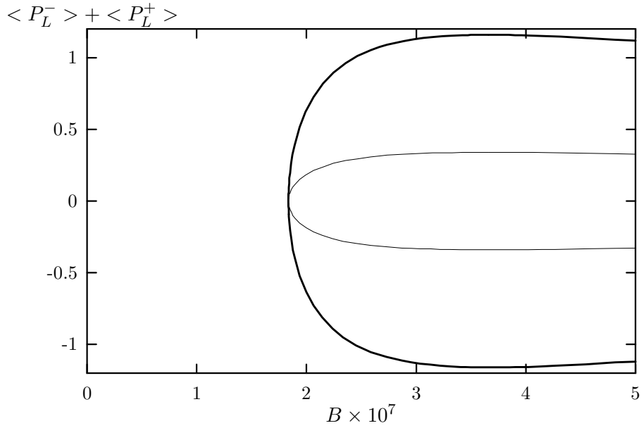
Figure 3: The flows in (\mathcal{B}, \langle P_L^- \rangle + \langle P_L^+ \rangle) plane. In each flow, C_{LRLR} + C_{LRRL} (thick solid line), C_{RLLR} + C_{RLRL} (thin line) are varied respectively.
