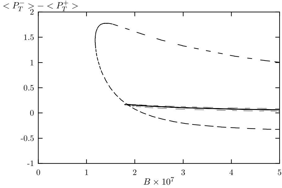
Figure 6: The flows in (\mathcal{B}, \langle P_T^- \rangle - \langle P_T^+ \rangle) plane. In each flow, C_{LRLR} + C_{LRRL} (thick solid line), C_{LRLR} - C_{LRRL} (thick dashed line), C_{RLLR} + C_{RLRL} (thick solid line), C_{RLLR} - C_{RLRL} (thin dashed line) are varied respectively.
