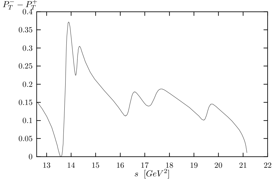
Figure 2: P_T^- - P_T^+ in the SM.
